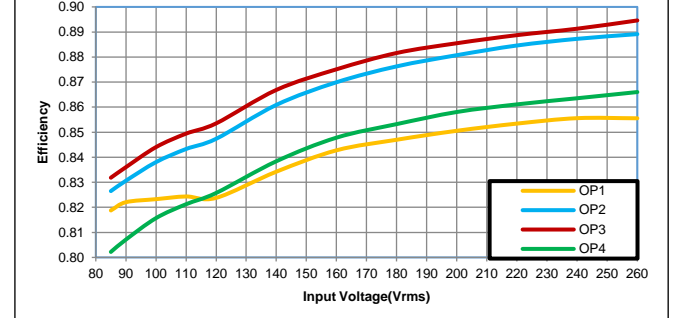
Typical Line Efficiency (Pmax)
