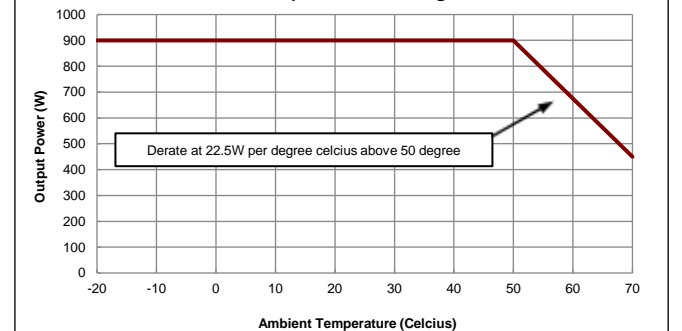
Temperature Derating
