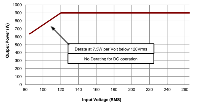
Line Derating
